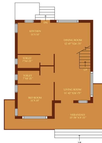
NARMADA (Ground Floor) 1,700 sq. ft.
